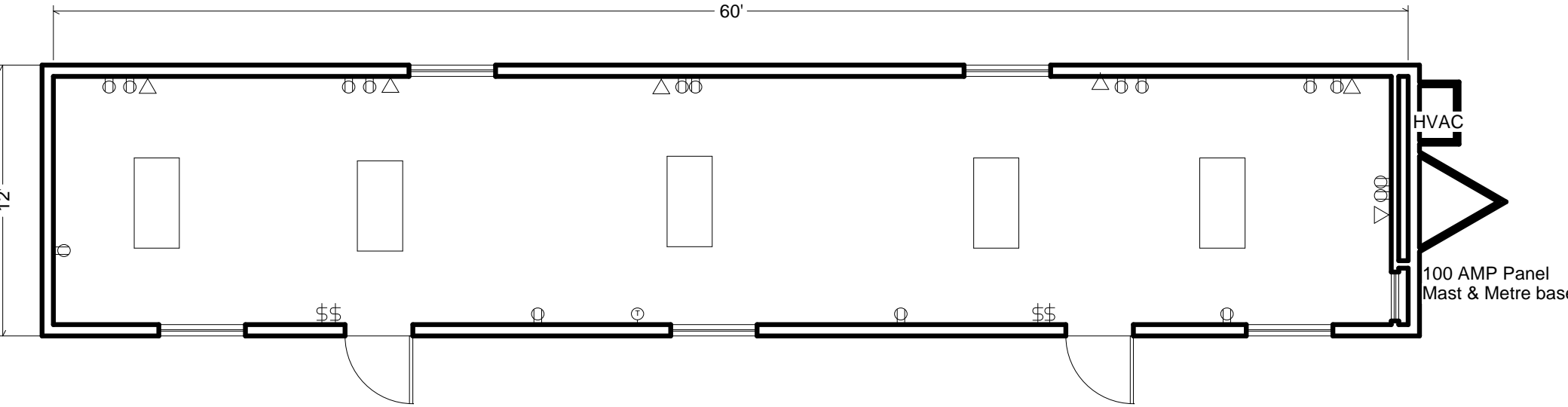
MOBILEASE 12x60' OFFICE TRAILER c/w Central HVAC
