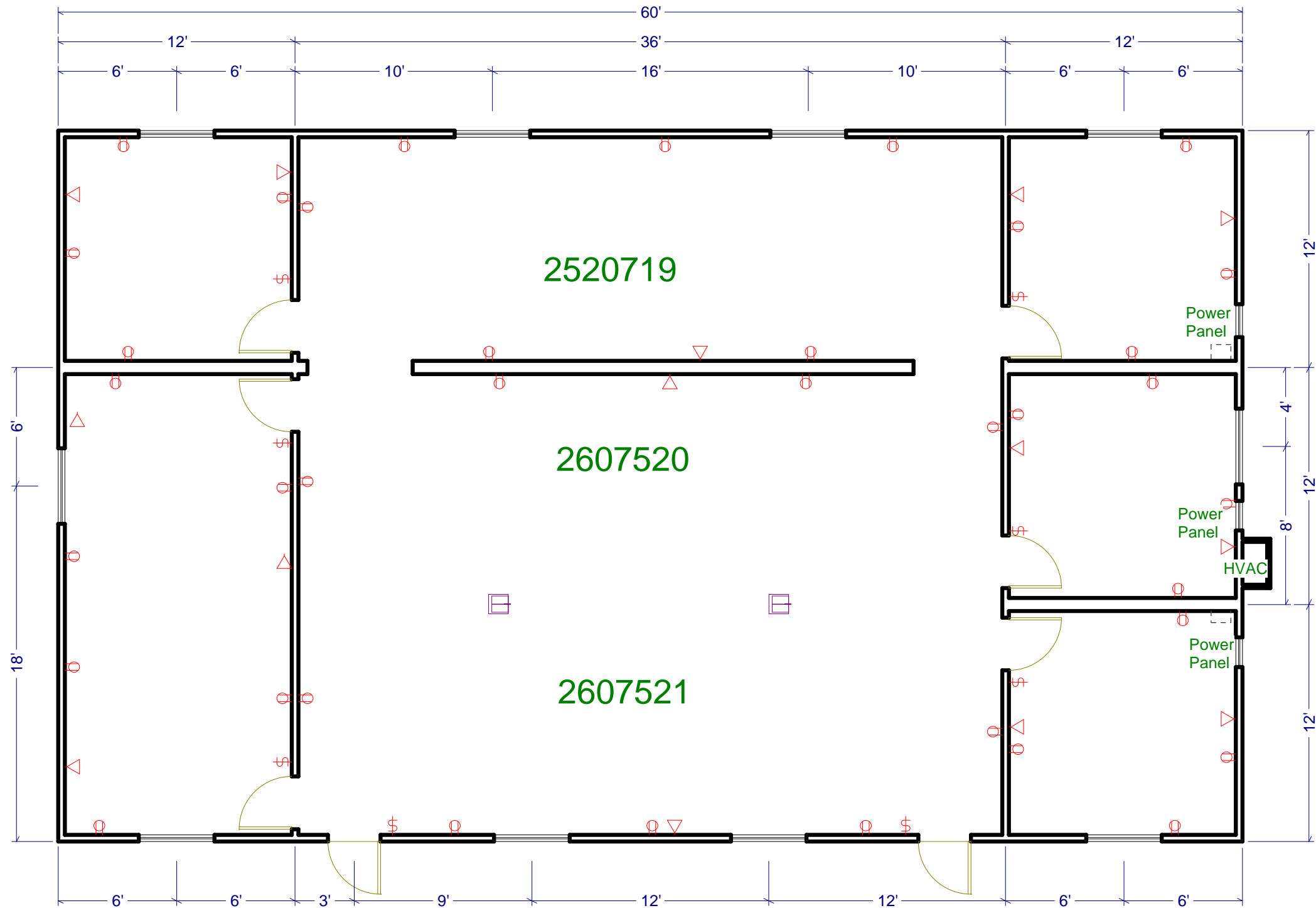
36X60' OFFICE COMPLEX - 6081 Royal BLUE FASCIA 4-12x12 Office, 1-12x24 Office
