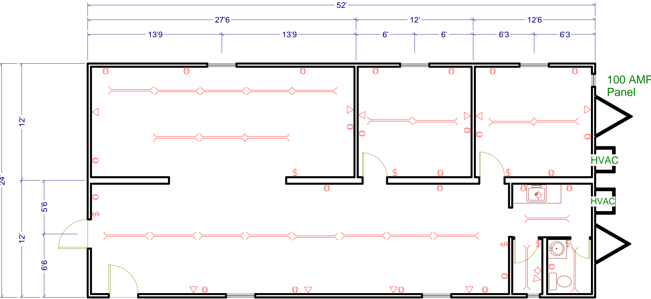
24x52' Office Complex
