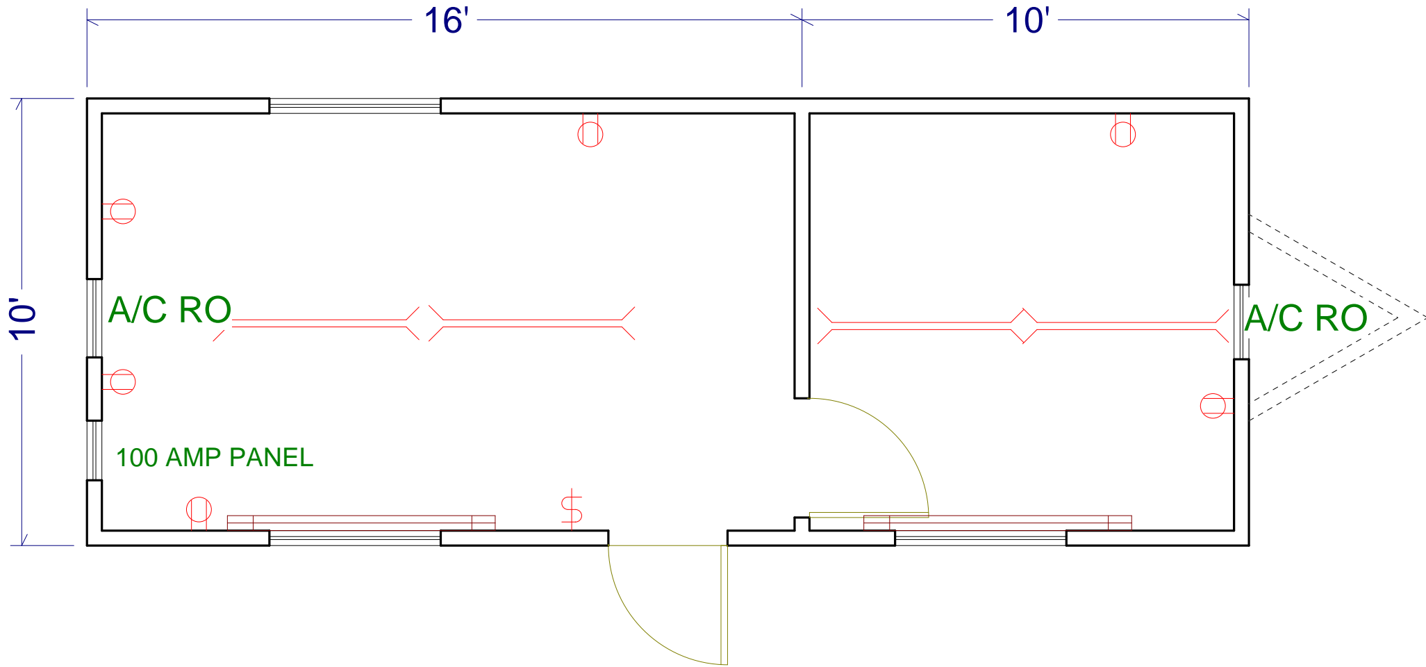
MOBILEASE 10x26' OFFICE TRAILER C/W 1 Partition
