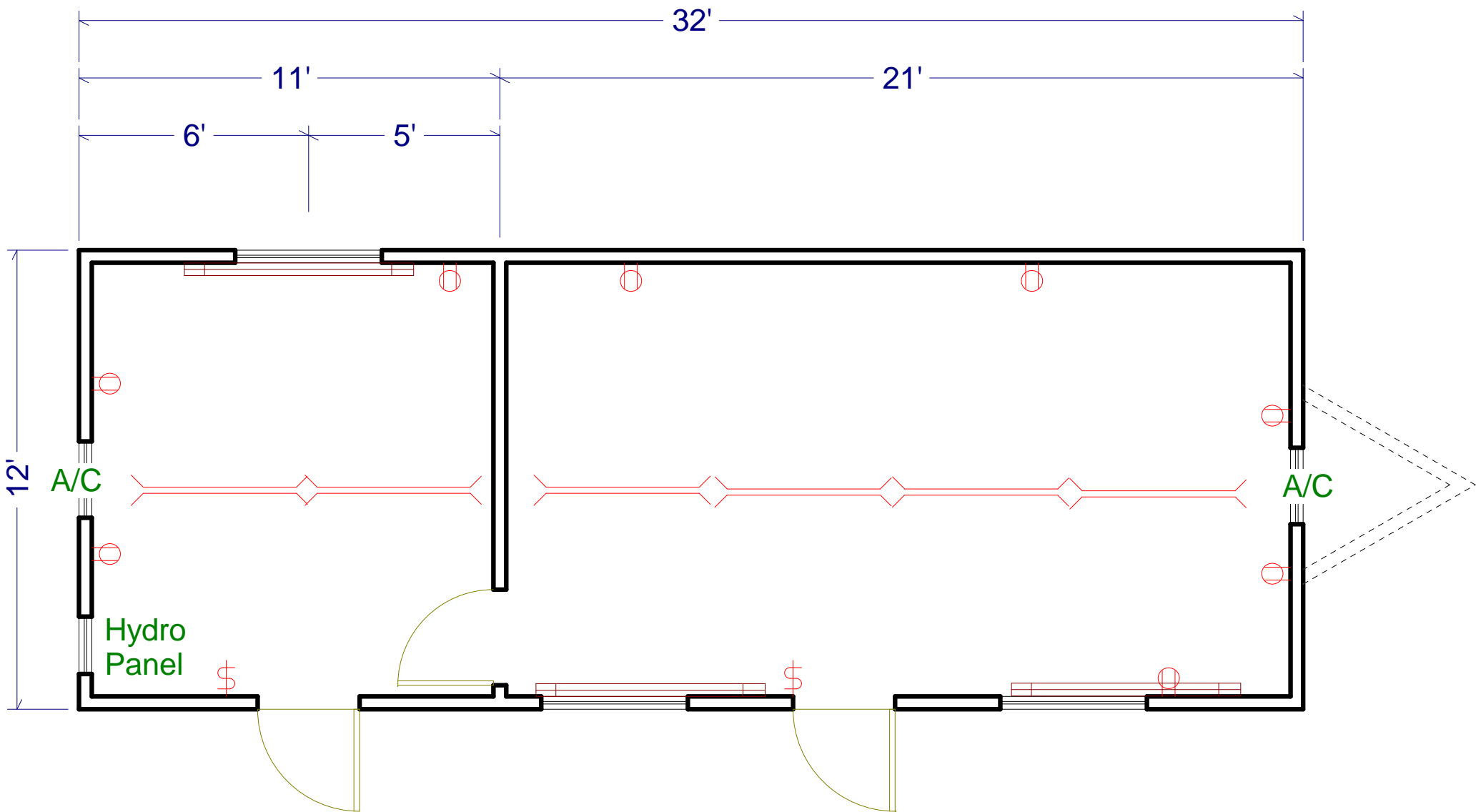
MOBILEASE 12x32' OFFICE C/W 1 Partition
